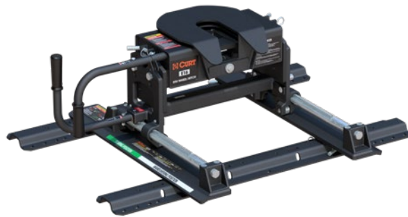
16616 - E16 head with R16 roller and base rails
