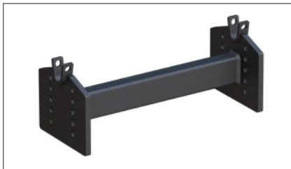
16505 head adapter allows CURT rollers to accept the 16515 E16 head (included in 16515, 16516 and 16616 kits)
