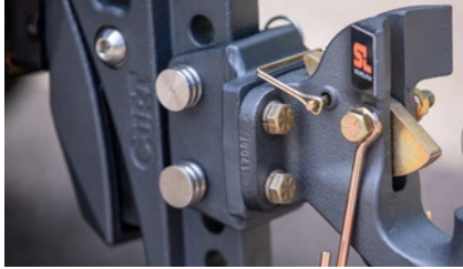
Pintle mount accepts any CURT mount-style pintle hook or ball & pintle hitch (45950)
