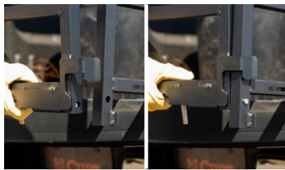
Innovative pin-latch system for fast installation and removal as needed. No drilling required
